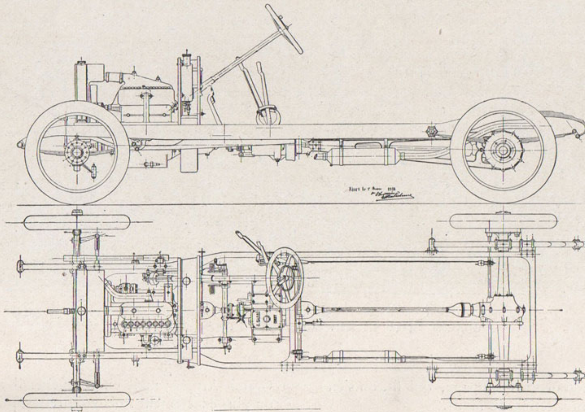
CHASSIS 10×12 HP BARRÉ 75×120, TYPE 1913
