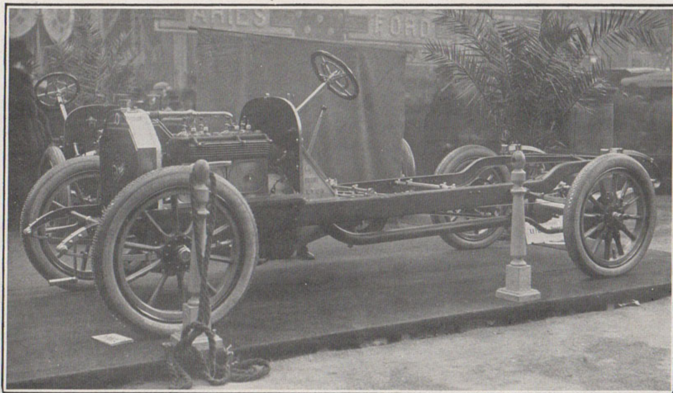
CHASSIS 12 HP LA BUIRE 4 CYLINDRES 80 \times 160
