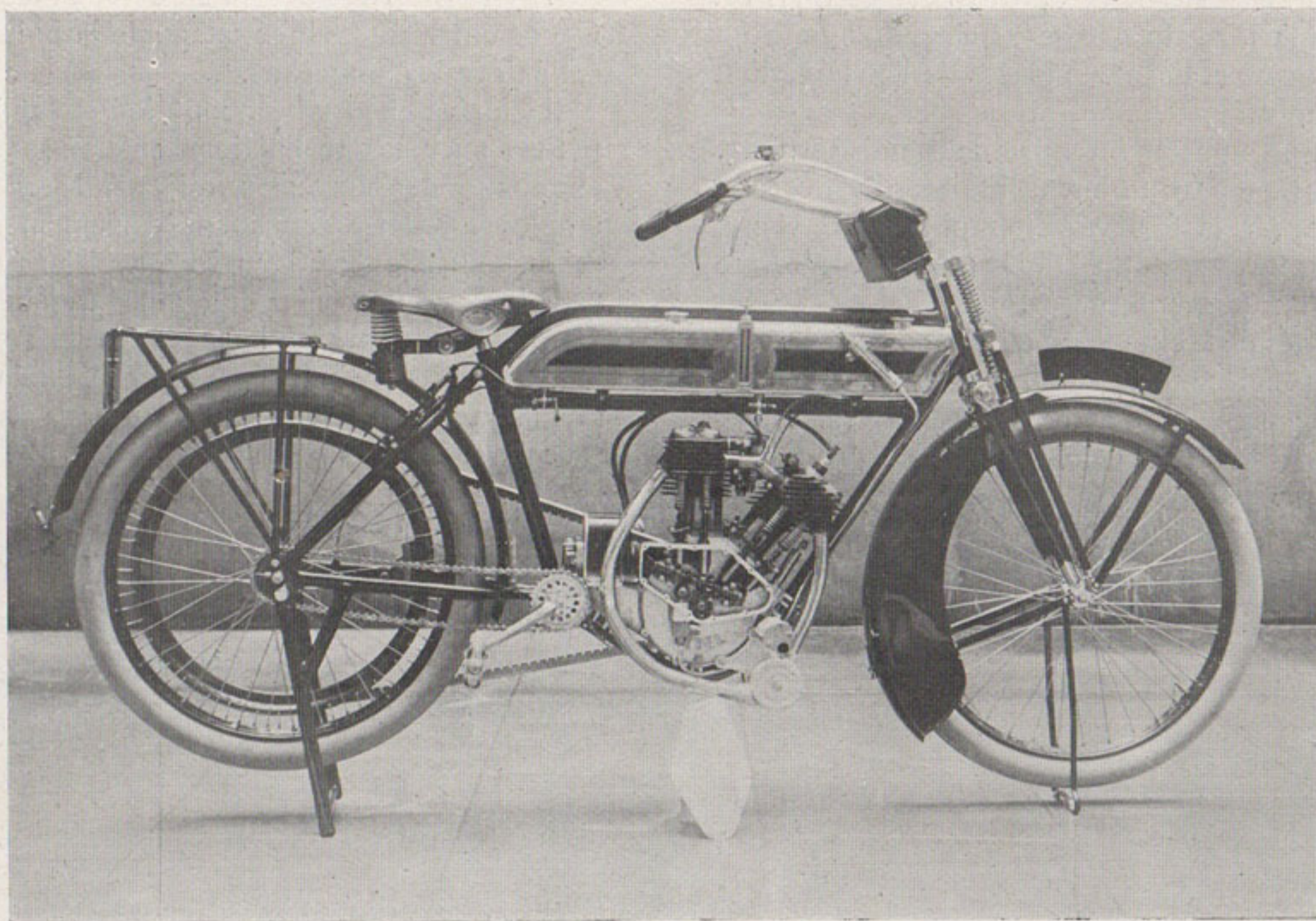
MOTORETTE TERROT, 4 1/2 HP 2 CYLINDRES 67 x 90
