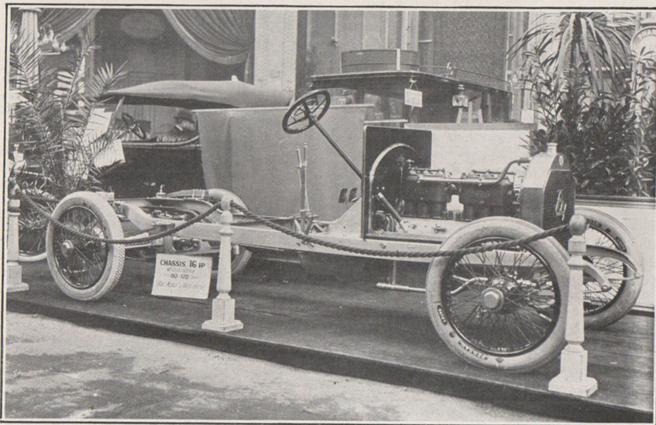
CHASSIS 16 HP MOTOBLOC 6 CYLINDRES 80 \times 120
