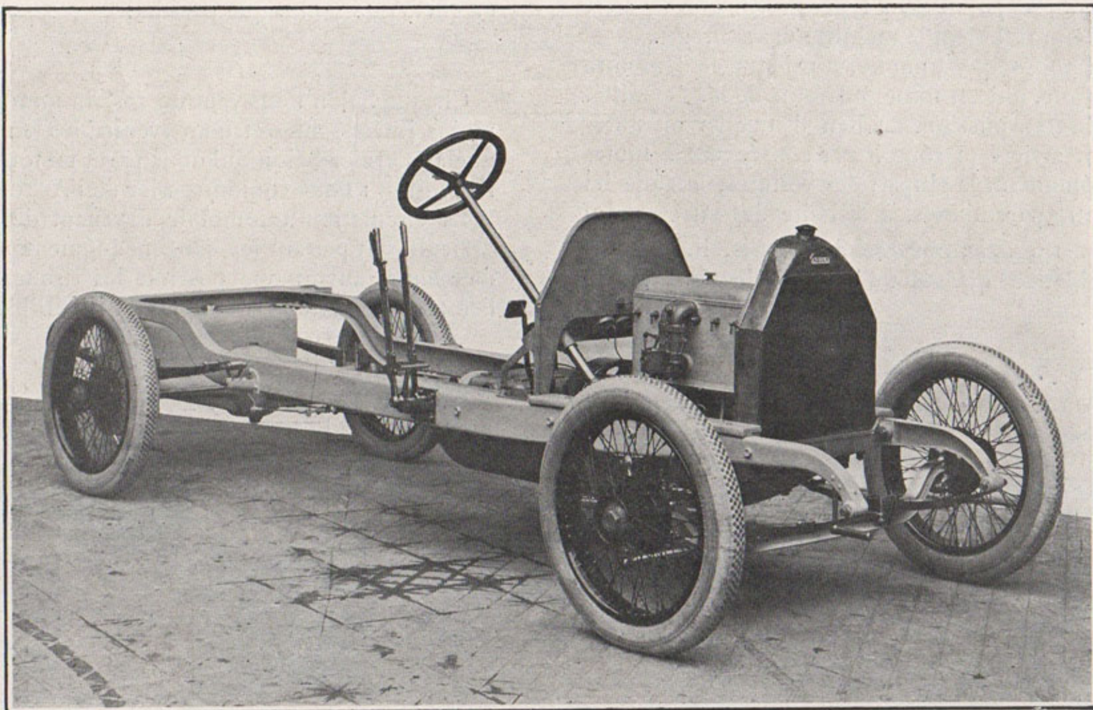
CHASSIS AQUILA ITALIANA 35-50 HP SIX CYLINDRES 80×130
