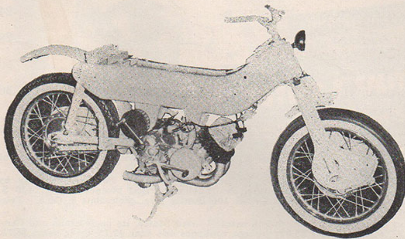
Under the smooth "skin" of the new Ariel is this massive box-section frame and compact twin cylinder power unit.
