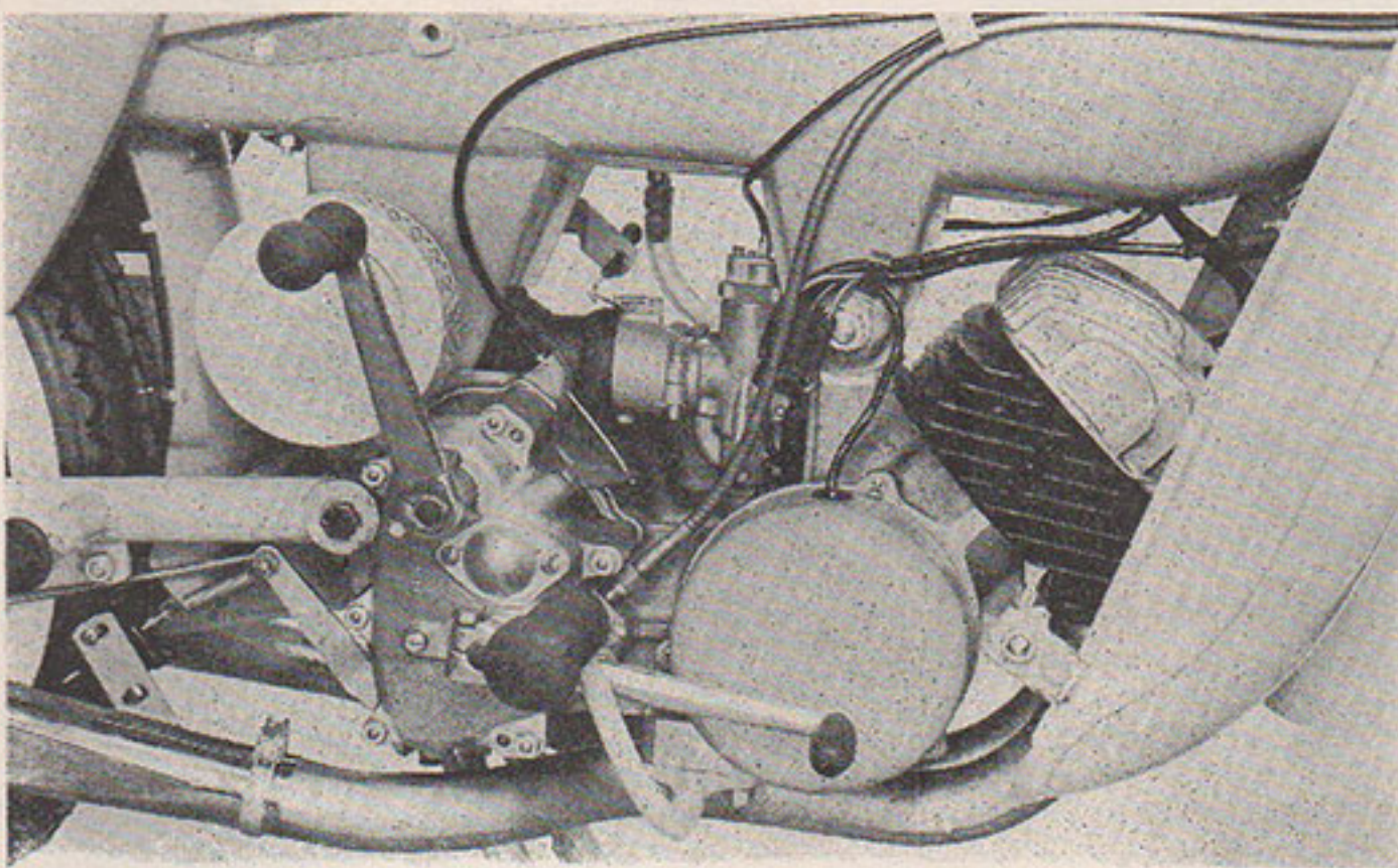
Quickly removable side panels give easy access to the "works". Note new air-flow cylinder fin design.
